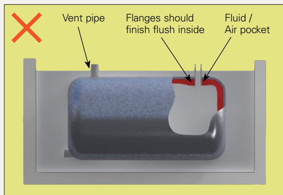
Figure 29: Hollow Vessels - Bad Design
